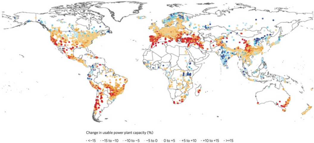
Figure 12 Future projection forecasts of annual usage of hydroelectric power plants due to climate-change and changes in water resource utilization in 2050 in RCP8.5 scenarios
