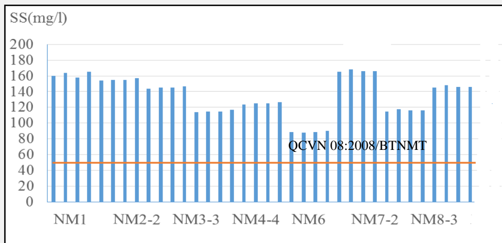
Figure 2 - 15: Suspended sediments concentration in the surface water samples
