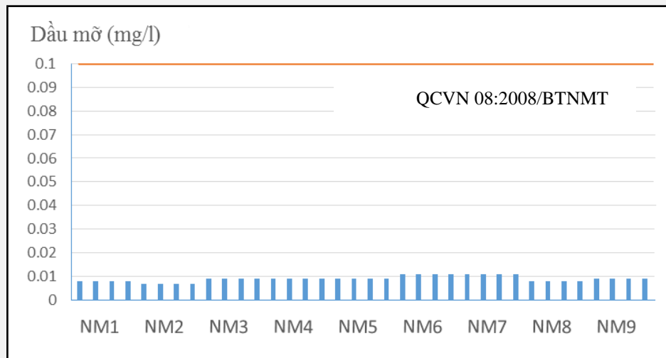
Figure 2 - 13: Oil concentration in the surface water samples
