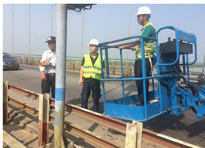
Installation of the inclinometer by using boomlift
