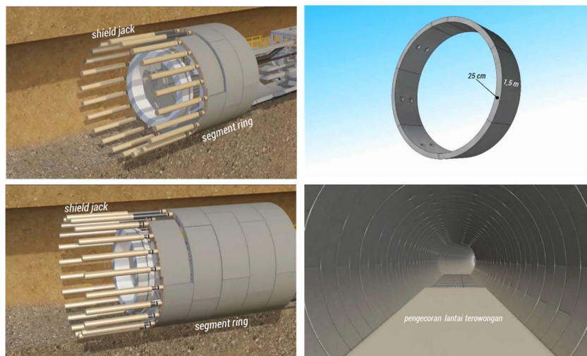
Figure 2.23. Illustration of Underground Tunnel Construction Work
