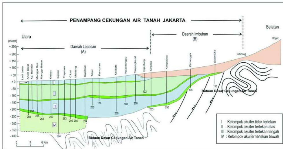
Figure 3.16. Jakarta CAT Zone
