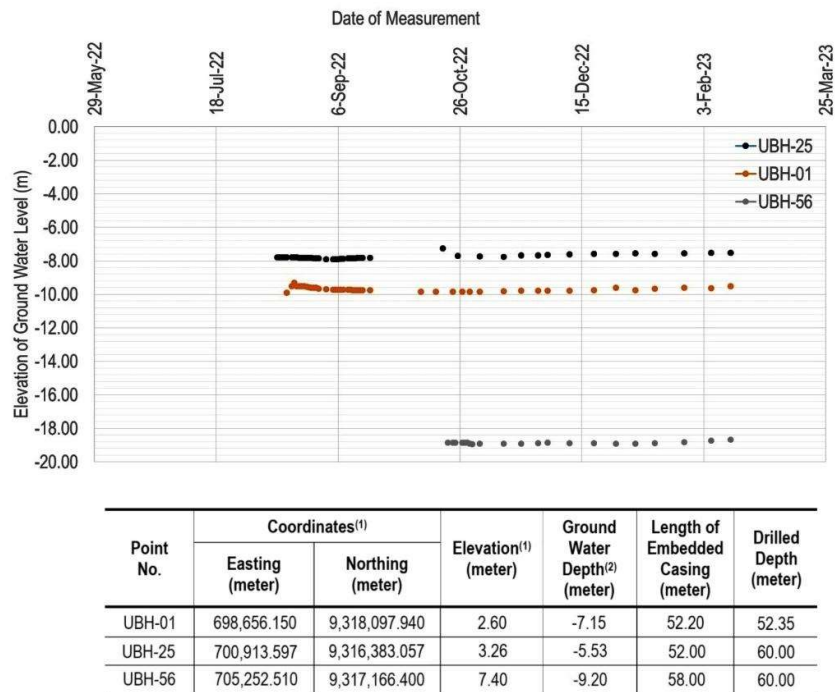
Figure 2.16. Groundwater Depth Profile
