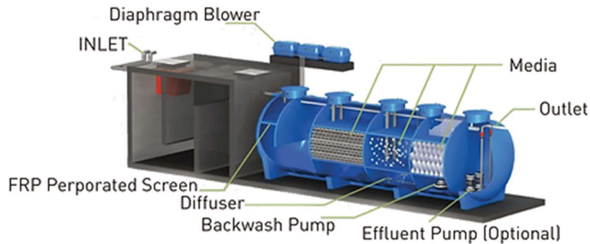
Figure 2.31. STP Anaerobic-Aerobic Biofilter System
