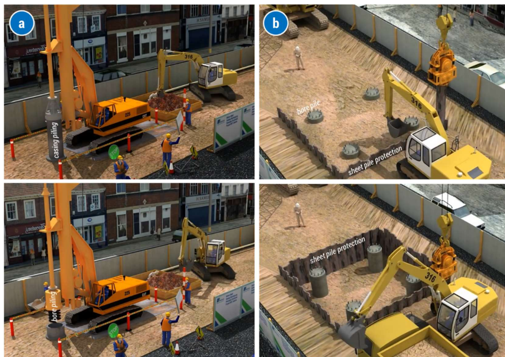
Figure 2.20. Illustration of Earthwork in Making Pier Foundations
