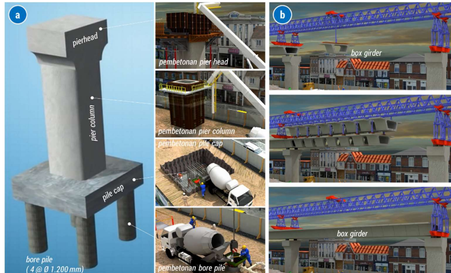
Figure 2.24. Illustration of Elevated Station Support Pole Construction
