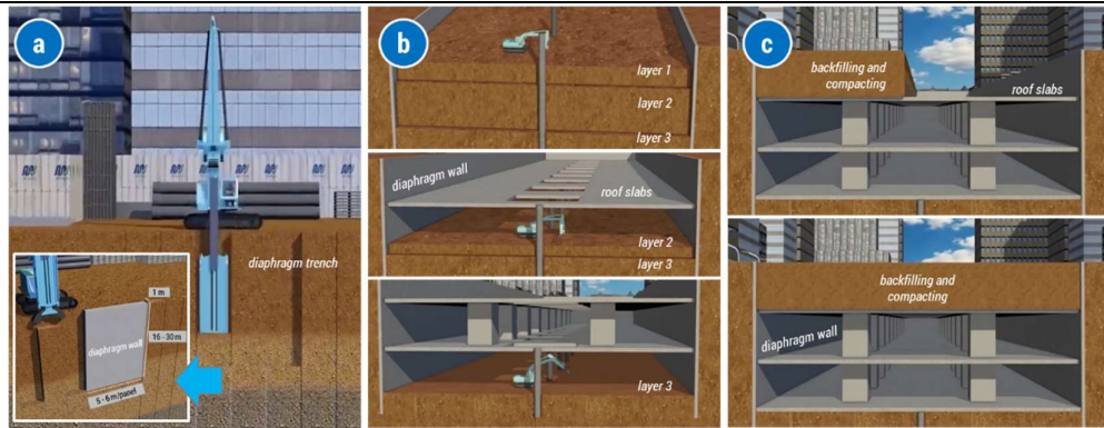
Figure 2.9. Illustration of Earthworks for Underground Station Construction
