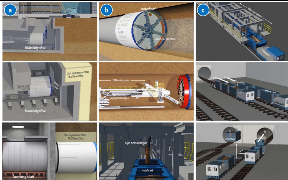
Figure 2.18. Illustration of Tunnel Excavation
