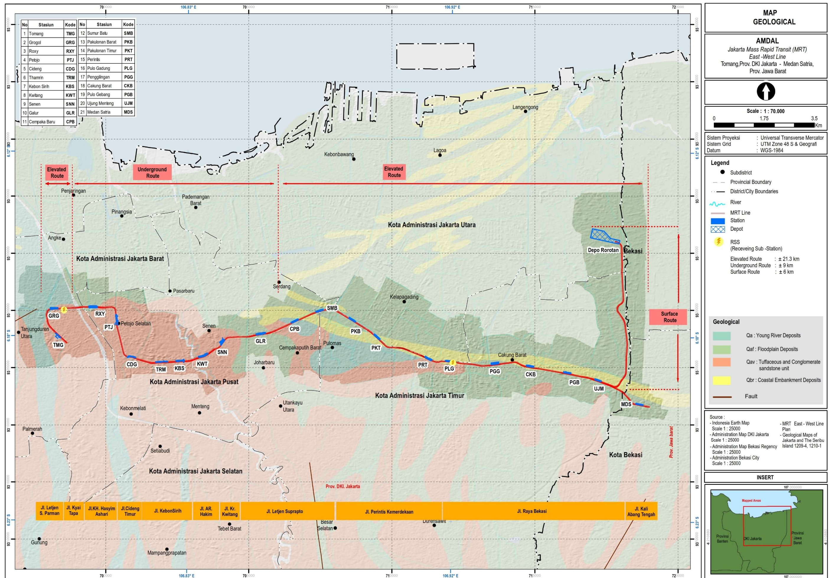
Figure 3.14. Geological Map of the Study Area Source: Regional Geological Map of Jakarta and the Thousand Islands (1992)
