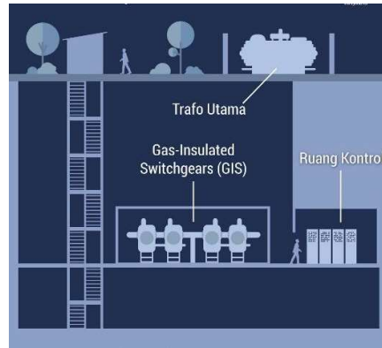
Figure 2.29. RSS illustration
