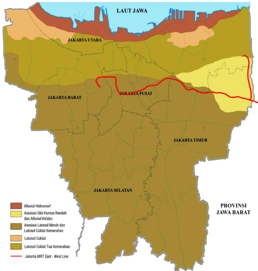
Figure 3.23. Soil Types in the Study Area
