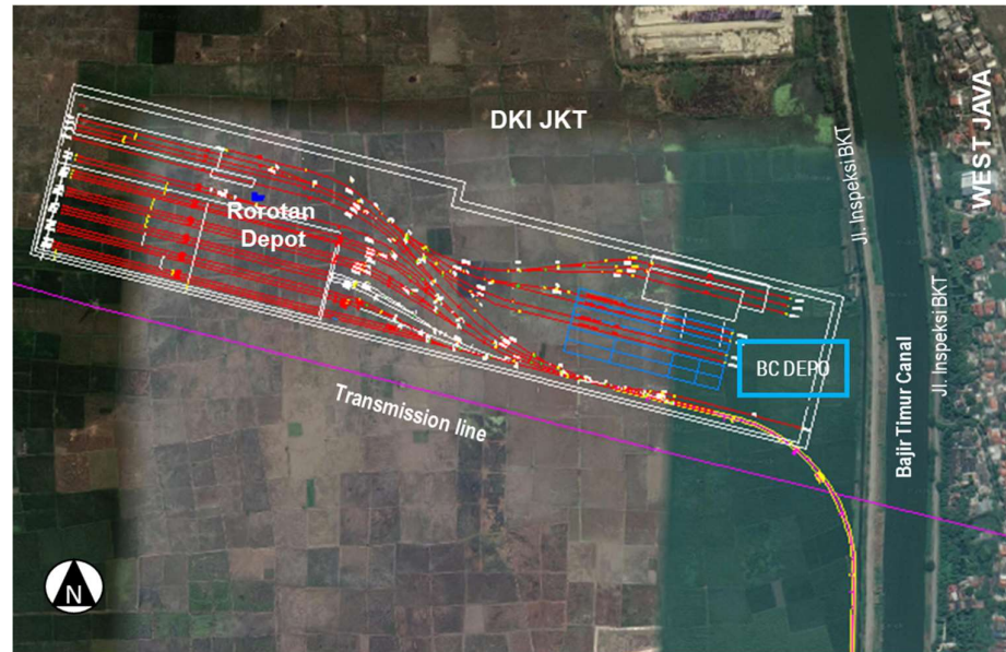
Figure 2.4. DEPO Basecamp Location Plan (Tentative)
