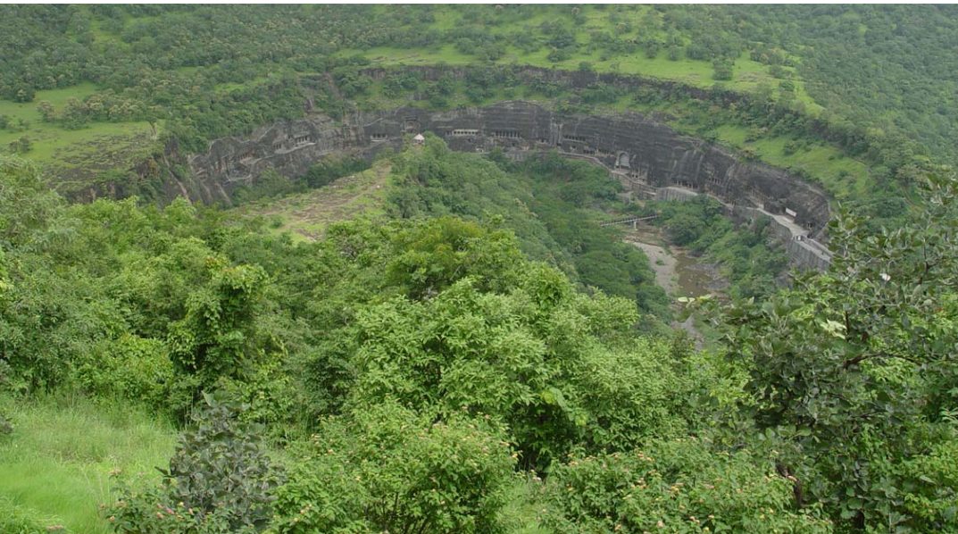
Afforested area that lies below Ajanta Viewpoint (left) and a view of the afforested area seen from the historic site (right)
