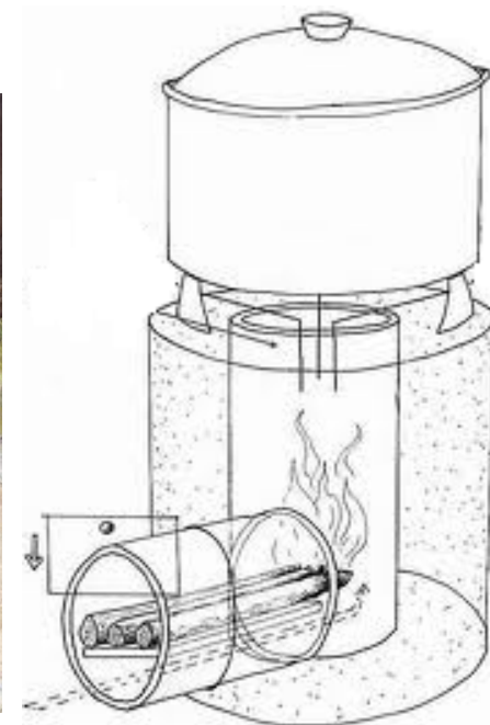
A rocket cooking stove newly installed
